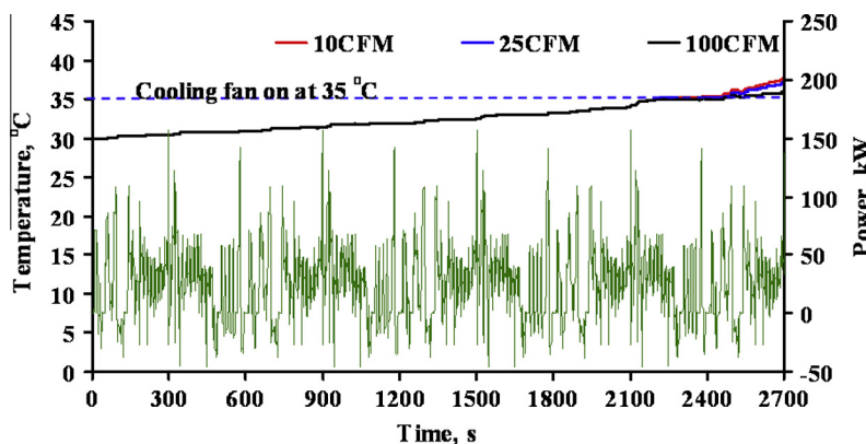
Fig. 10. Thermal response of 38,120 battery pack under US06 driving cycle.
